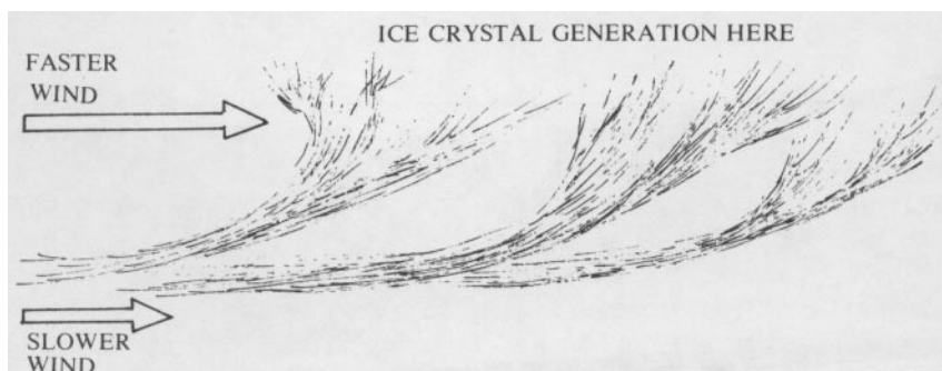
Figure 28 - Cirrus Clouds
