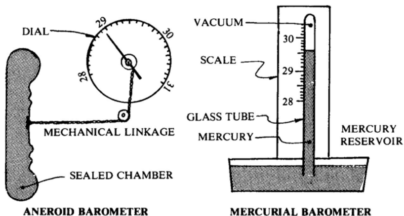
Figure 3 - Barometers
