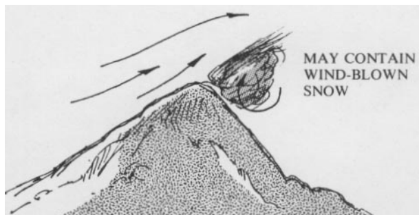
Figure 32 - Banner Cloud
