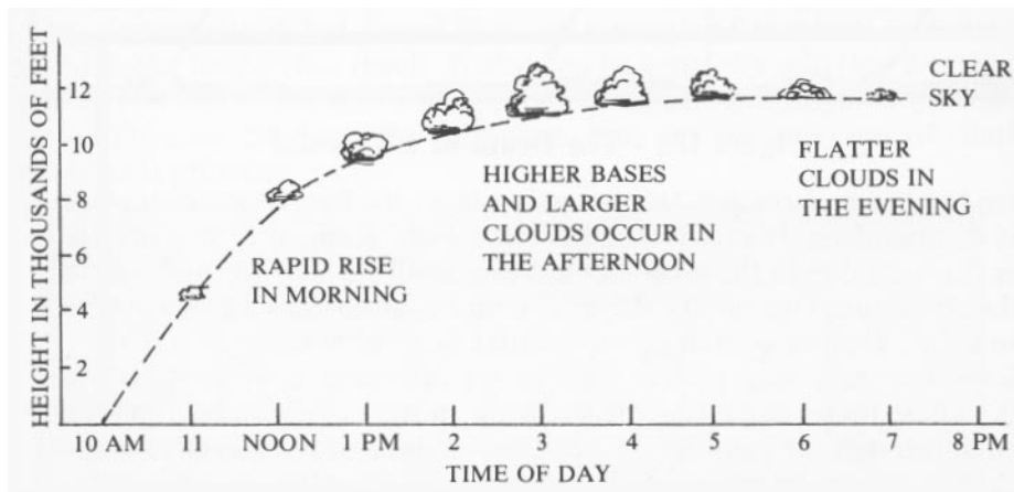
Figure 186 - Daily Thermal Height and Size Changes
