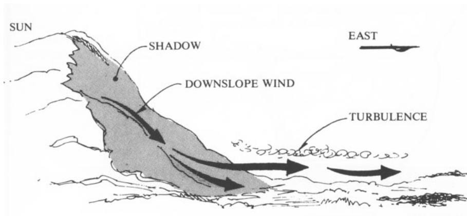
Figure 102 - Shear Caused by Downslope Winds
