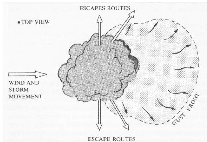
Figure 219 - Escaping a Thunderstorm
