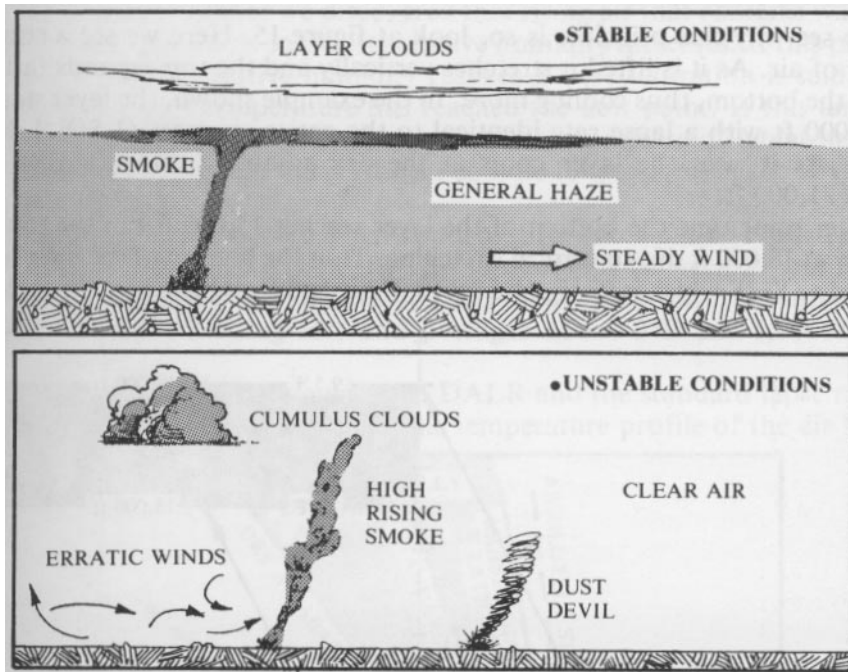
Figure 14 - Stability Indications
