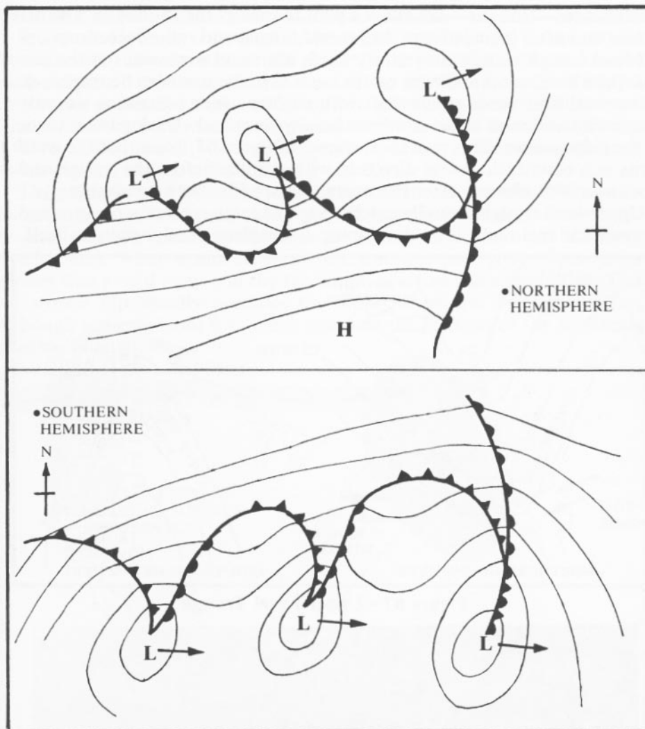
Figure 66 - Surface Waves
