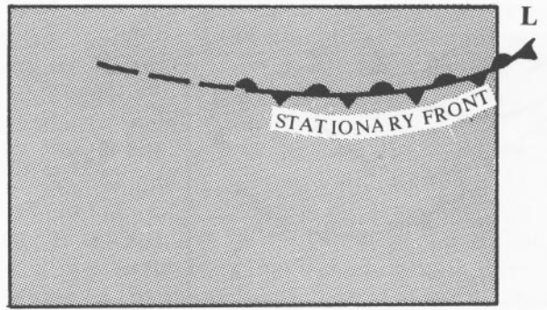
Figure 49 - Stationary Front
