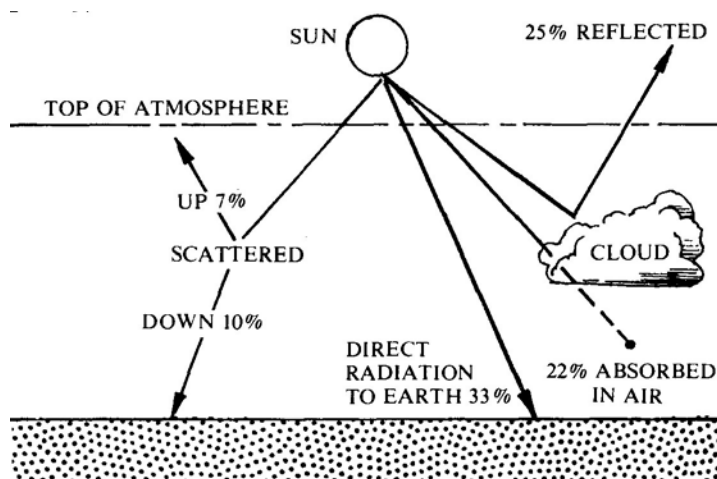
Figure 5 - Solar Heating
