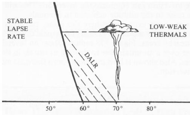
Figure 179 - Weak Thermals on a Stable Day
