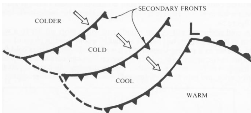
Figure 52 - Secondary Fronts
