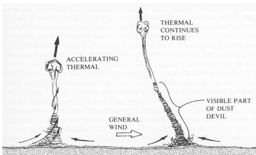
Figure 181 - Thermals Creating Dust Devils
