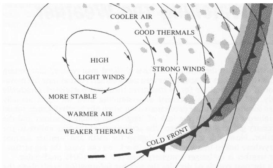
Figure 220 - Post-Frontal Conditions
