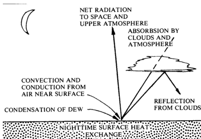
Figure 6 - Heat Radiation
