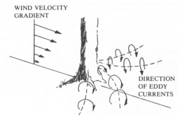
Figure 116 - Turbulence Downwind From a Tree
