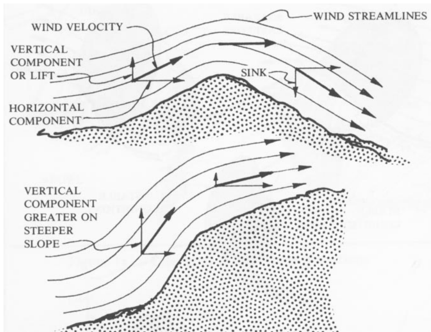
Figure 138 - Variations in Ridge Lift
