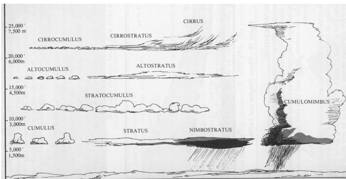
Figure 29 - Cloud Types and Altitudes
