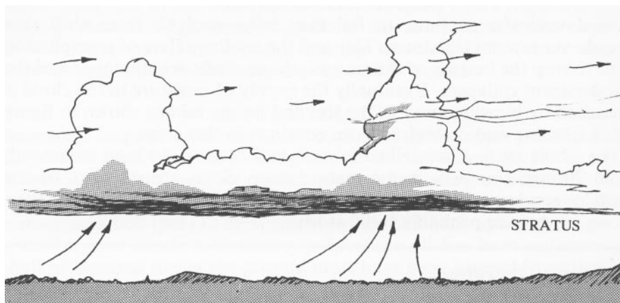
Figure 213 - Imbedded Thunderstorms
