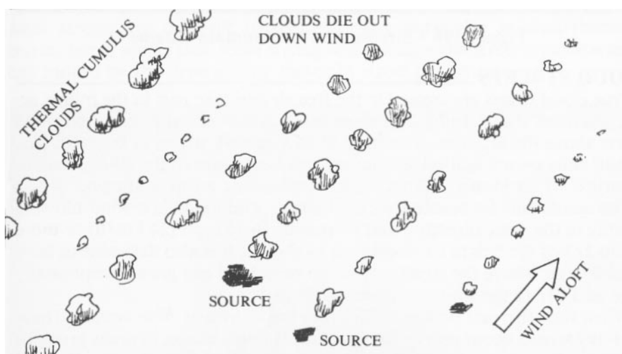
Figure 197 - Cloud Streams
