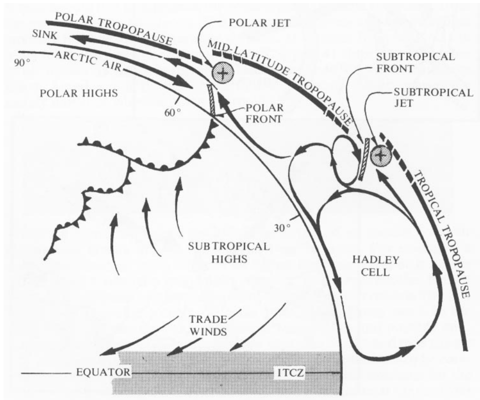
Figure 43 - The Lower Atmosphere in Cross Section
