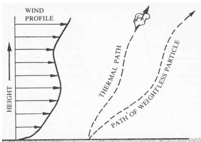
Figure 187 - Thermal Drifting in Wind
