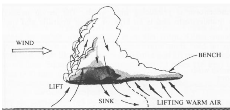
Figure 216 - Production of a Thunderstorm Bench
