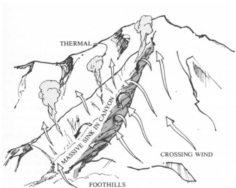
Figure 114 - High Mountain Canyon Flow
