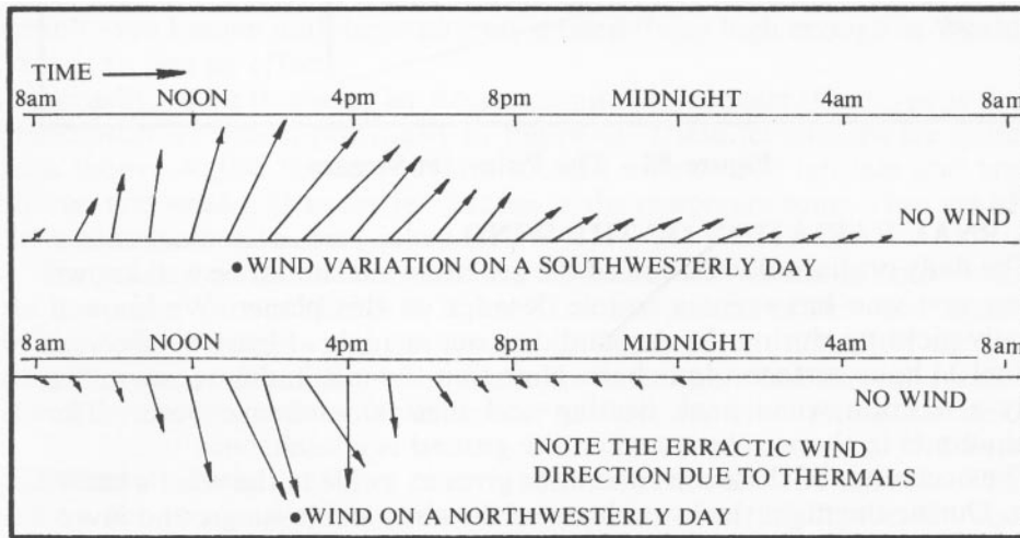
Figure 86 - Daily Wind Variation
