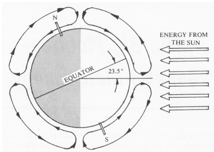
Figure 39 - General Circulation
