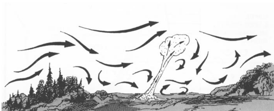
Figure 98 - Thermal Disruption of the Airflow
