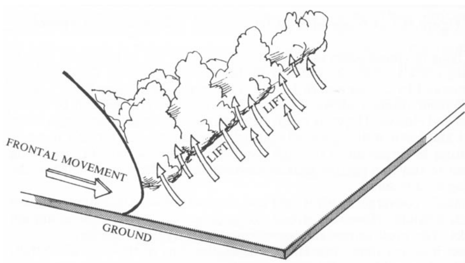
Figure 164 - Frontal Lift
