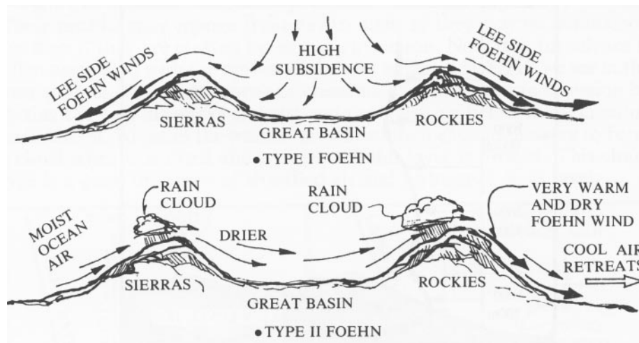
Figure 90 - Types of Foehn Winds
