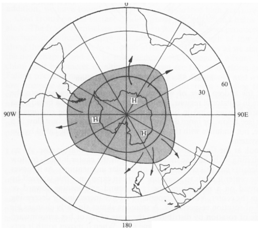
Figure 57 - Antarctic Air Masses
