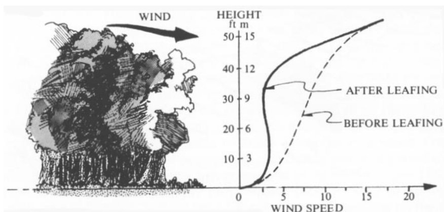
Figure 117 - Wind Shadow Due to Trees
