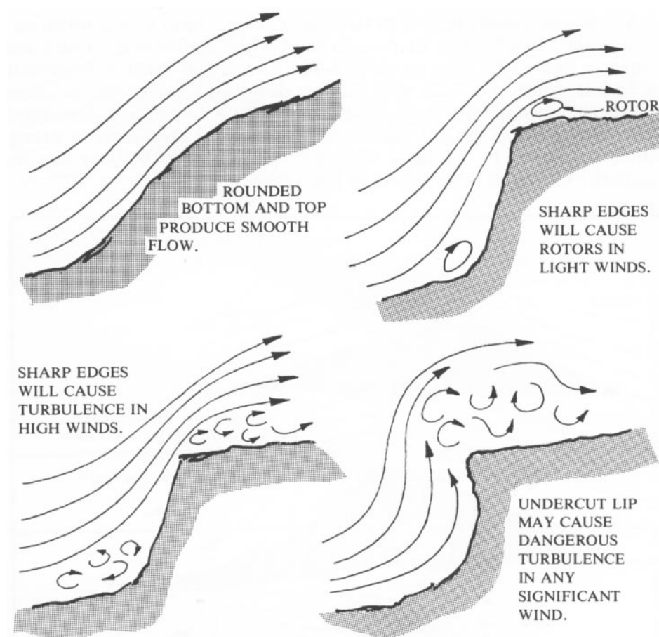
Figure 106 - Turbulence Near Hill Faces
