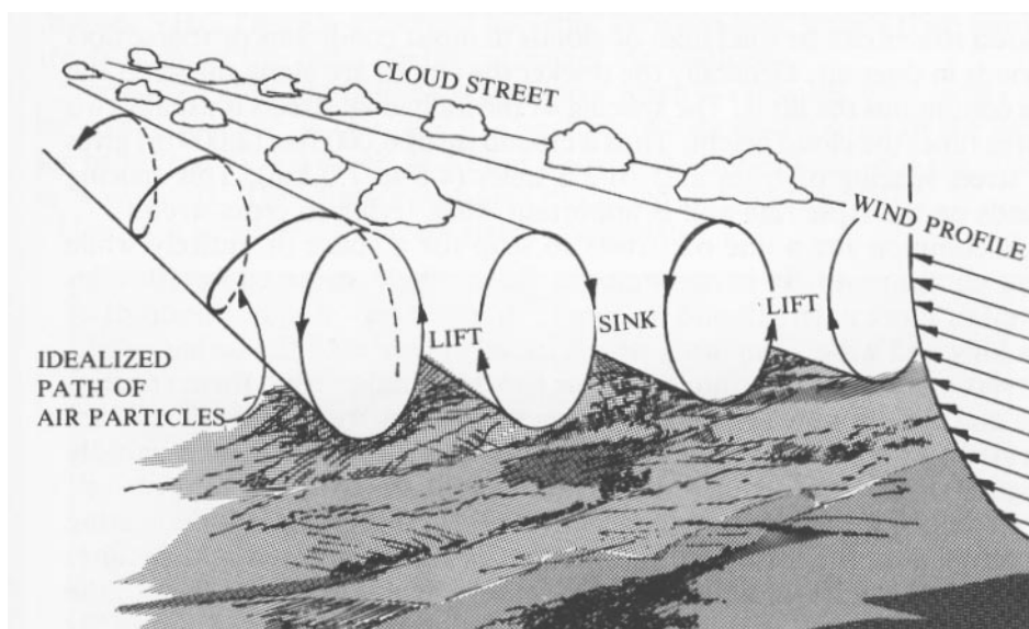
Figure 199 - Cloud Street Mechanics
