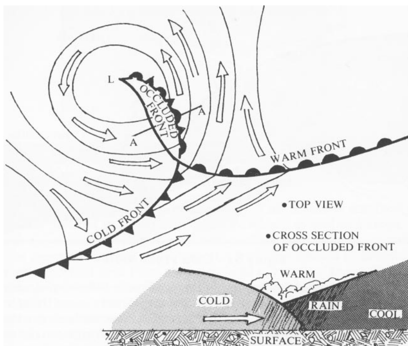
Figure 53 - Occluded Front
