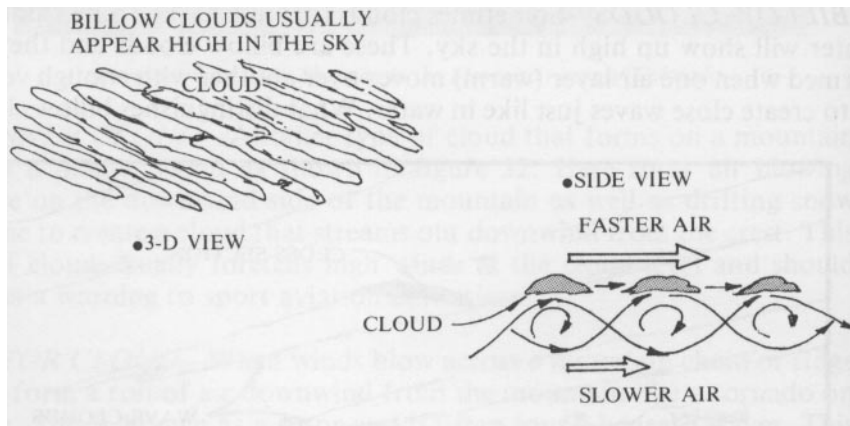
Figure 34 - Billow Clouds
