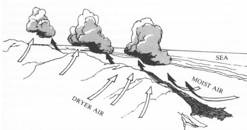
Figure 163 - Clouds with Different Bases Indicating Convergence
