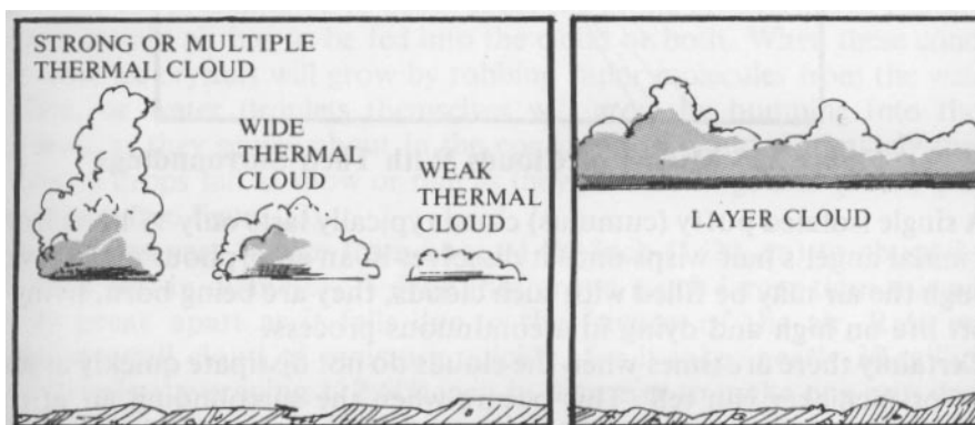
Figure 21 - Cloud Tops
