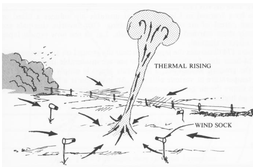
Figure 172 - Variable Ground Winds Under a Thermal
