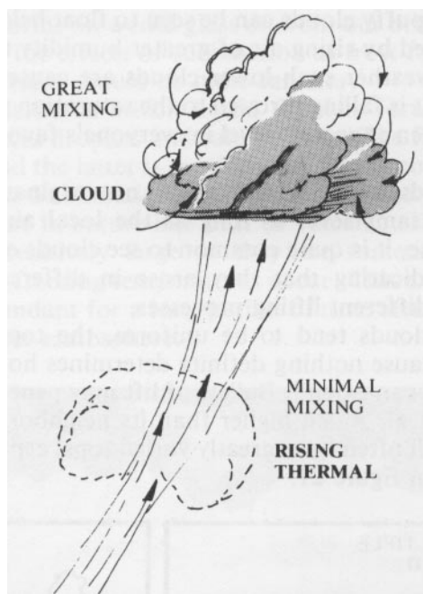
Figure 22 - Mixing of Clouds With Their Surroundings
