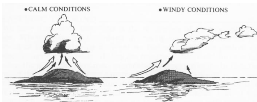
Figure 72 - Island Conditions
