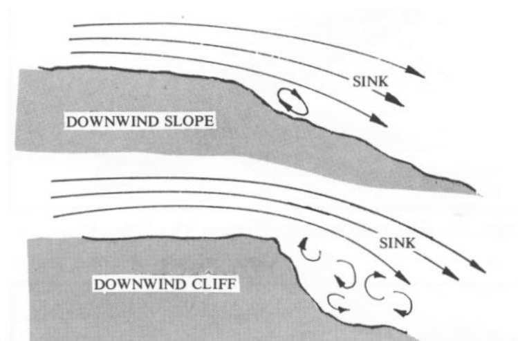
Figure 110 - Turbulence Downwind of a Plateau
