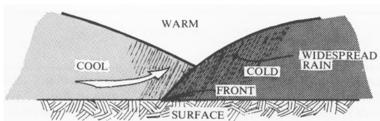
Figure 54 - Cross Section of Warm Occlusion
